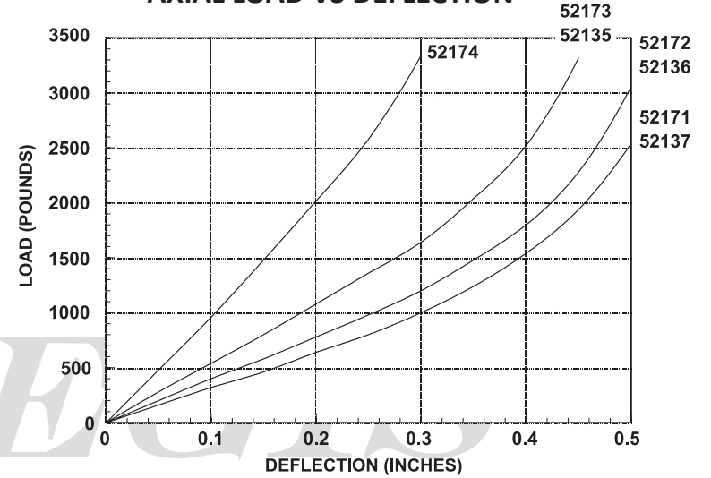
AXIAL LOAD VS DEFLECTION
