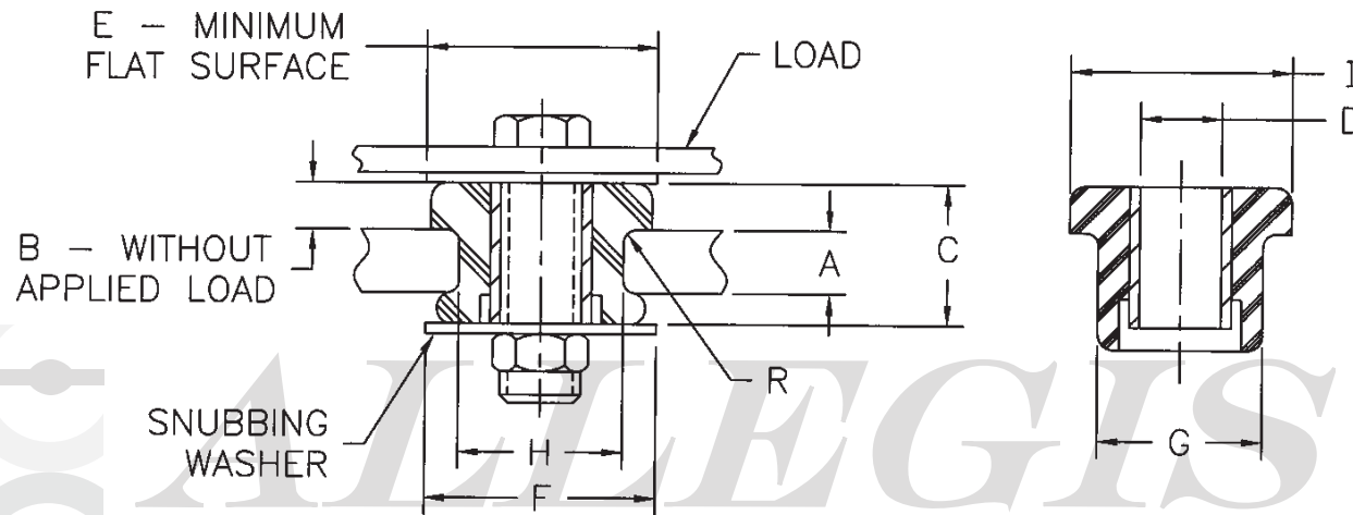
TYPICAL INSTALLATION
