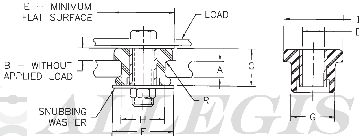
TYPICAL INSTALLATION
