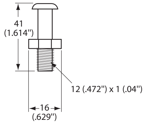
Striker Bolt (SOLD SEPARATELY)
