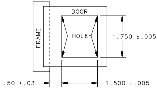
PANEL PREPARATION SCALE 1:2
