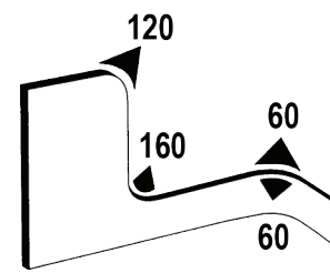
Bend Radius
