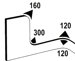
Bend Radius
